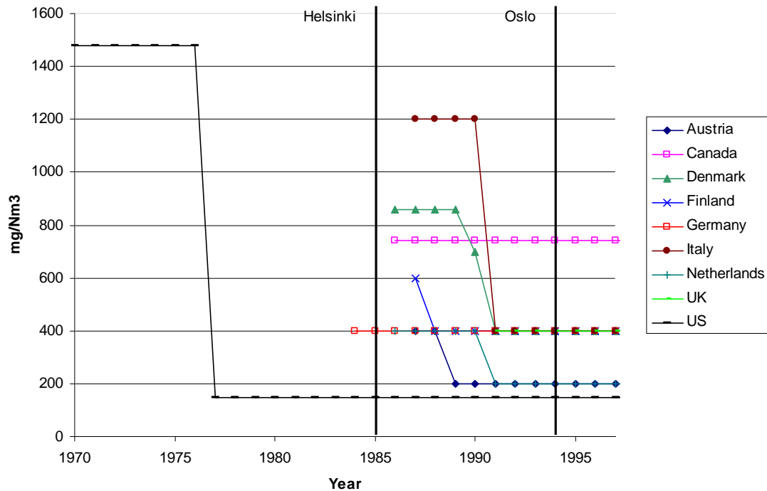
Figure 1: Regulatory standards for coal fired power plants (in \mu\text{g}/\text{Nm}^3 )
